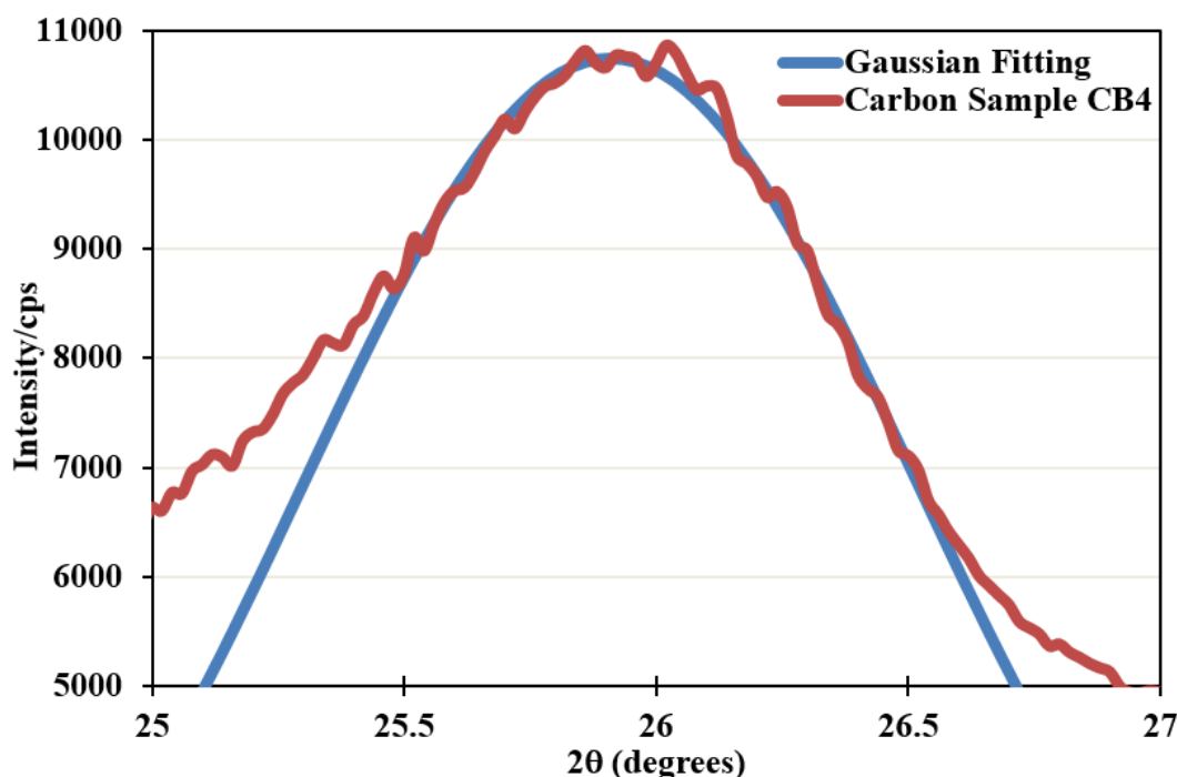
Fig. 10. The relatively most intense XRD peak of carbon sample CB4 appeared at 2\theta = 26.04^\circ . The FWHM value is mentioned in the inset
