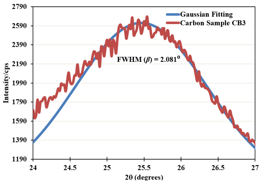
Fig. 9. The broad yet relatively more intense XRD peak of carbon sample CB3 appeared at 2\theta = 25.54^\circ . The FWHM value is mentioned in the inset
