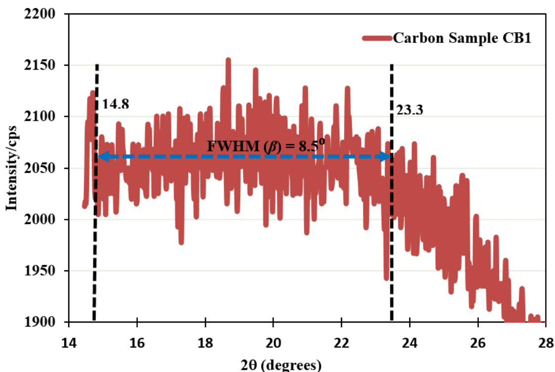
Fig. 7. The diffusive XRD peak of carbon sample CB1 protruded at 2\theta = 19.48^\circ . The manually calculated FWHM value is mentioned in the inset (the Gaussian convolution peak fitting technique was impracticable due to extreme peak-broadening and obtuseness)
