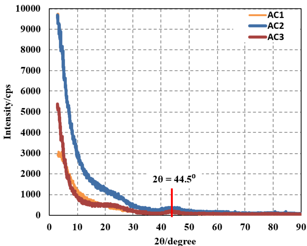
Fig. 1. The X-ray diffraction spectra for activated carbon samples AC1, AC2, and AC3 carbonized at \sim 600\text{--}900^\circ\text{C}
