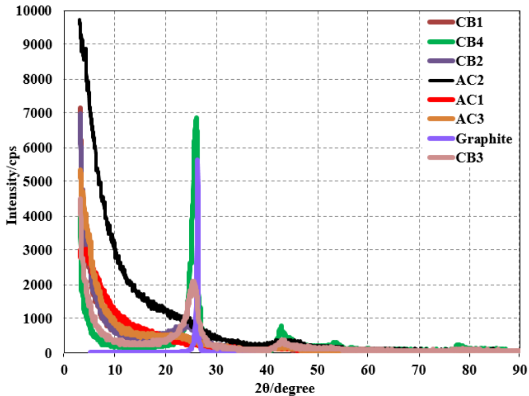
Fig. 6. Comparison of the XRD patterns of the carbon materials heated at different temperature regimes. The diffraction datasets for the most intense XRD band ( 2\theta = 26.7^\circ ) of the graphite are also plotted for the comparison purpose
