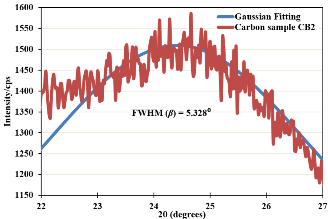
Fig. 8. The broad yet relatively intense XRD peak of carbon sample CB2 appeared at 2\theta = 24.66^\circ . The FWHM value is mentioned in the inset
