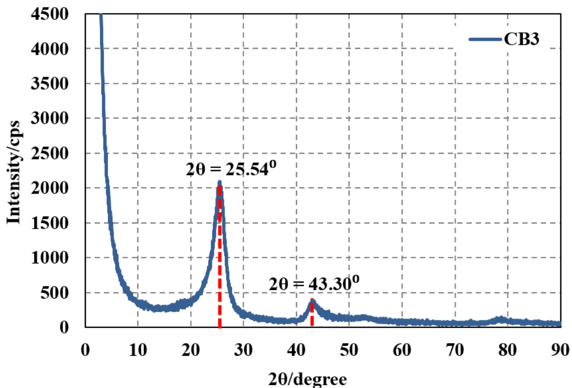
Fig. 4. The X-ray diffraction spectrum for carbon clack CB3 graphitized at ~2000°C
