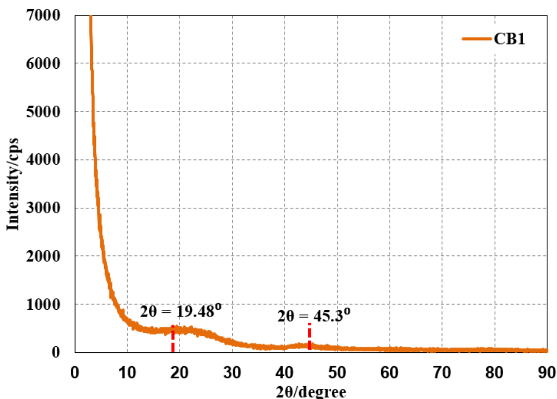
Fig. 2. The X-ray diffraction spectrum for carbon black CB1 carbonized at \sim 800^\circ\text{C}
