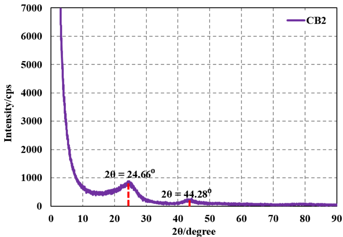
Fig. 3. The X-ray diffraction spectrum for carbon clack CB2 graphitized at ~1400°C
