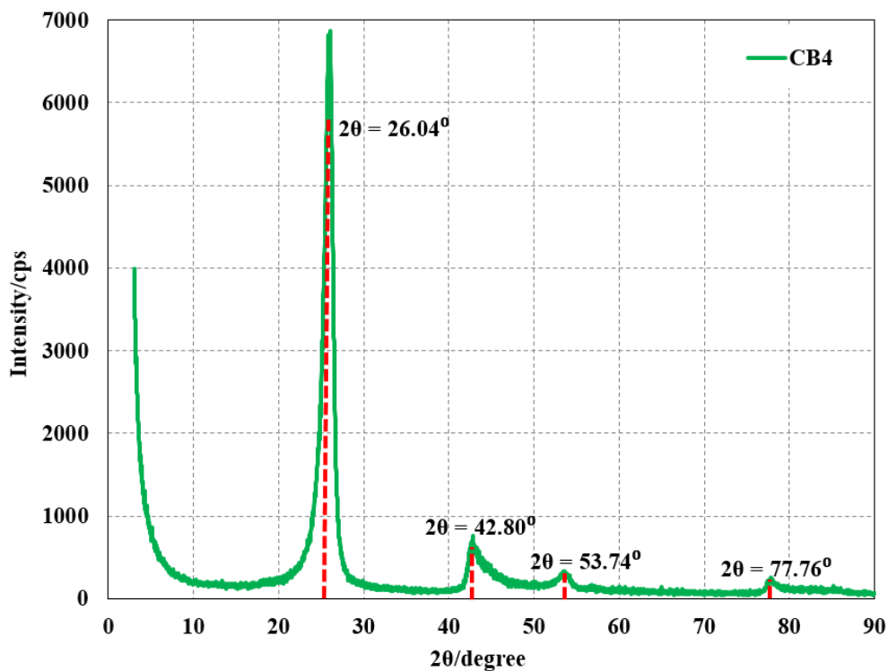
Fig. 5. The X-ray diffraction spectrum for carbon clack CB4 graphitized at > 2500°C
