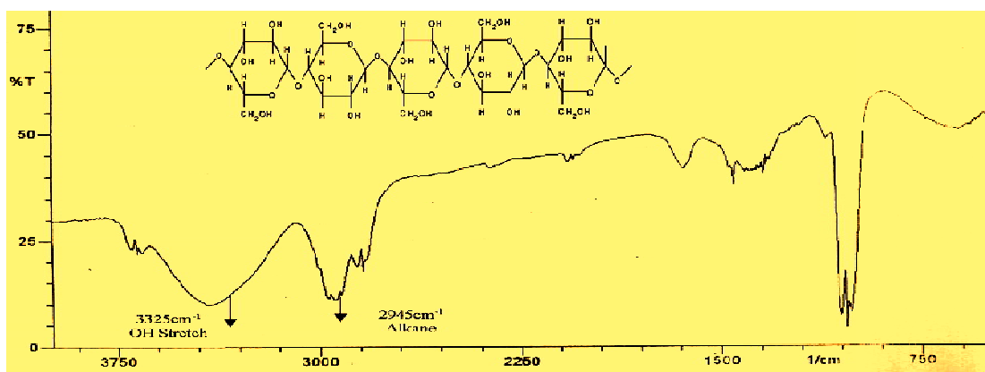
Fig. 5. FT-IR spectrum of the distillate obtained from fermented banana peels
