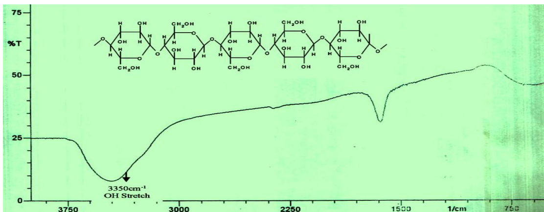
Fig. 6. FT-IR spectrum of the distillate obtained from fermented plantain peels
