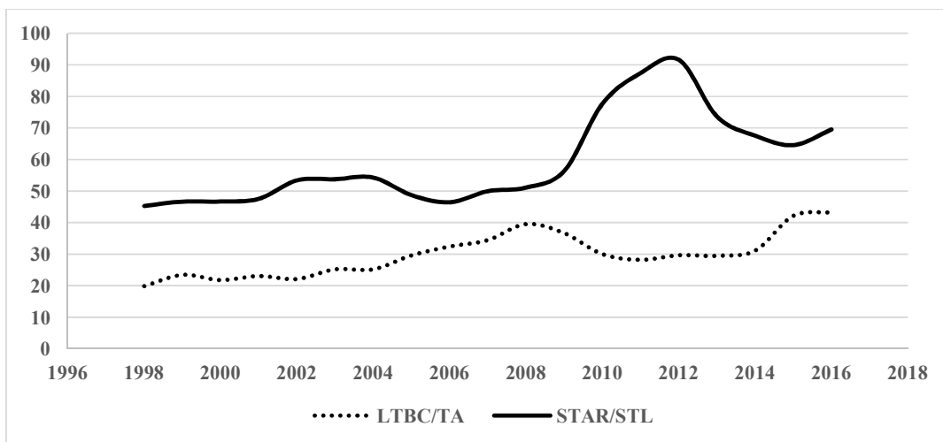
Fig. 1. LTBC/TA and STAR/STL in forestry products sector in Turkey (1998 – 2016)
