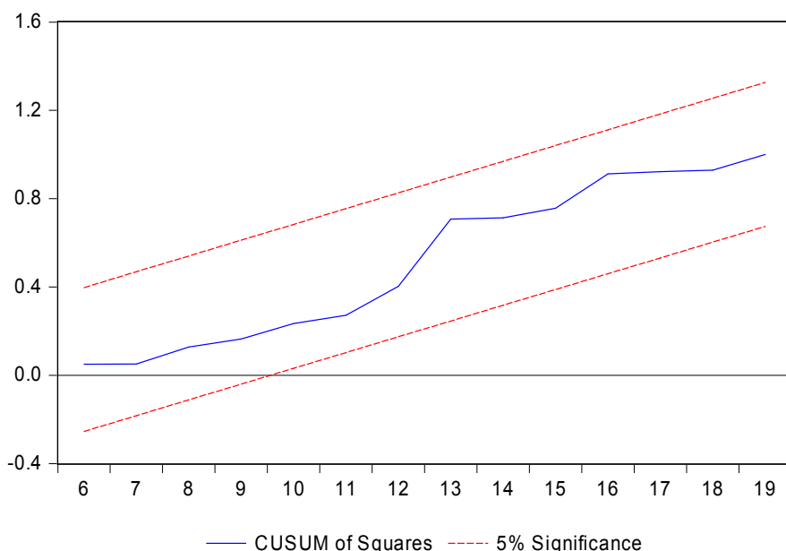
Fig. 4. CUSUM test for the Model B
