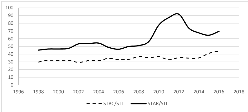
Fig. 2. STBC/STL and STAR/STL in forestry products sector in Turkey (1998 – 2016)
