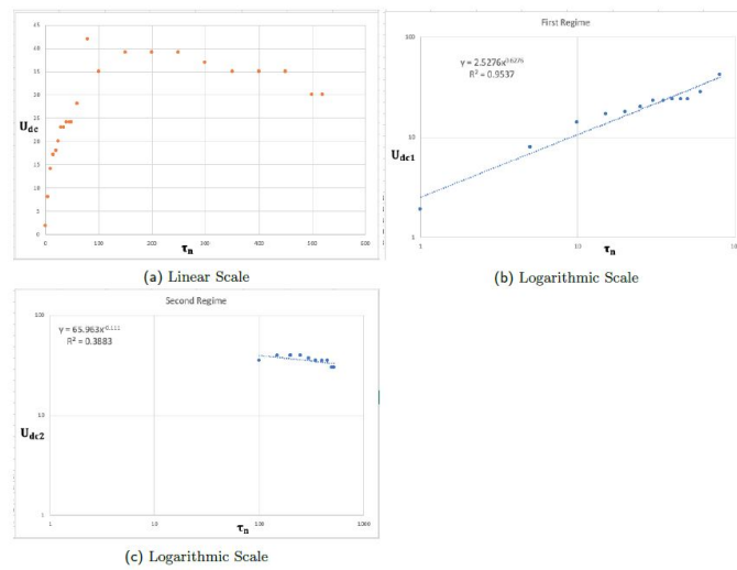
Fig. 11. Propagation speed of the Density current U_{dc} for the different Regimes with respect to time \tau_n at barrier position 1.12L/14 .
