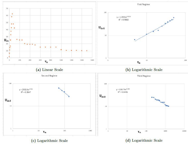
Fig. 4. Propagation speed of the Density current U_{dc} for the different Regimes with respect to time \tau_n at barrier position 0.14L/14 .
