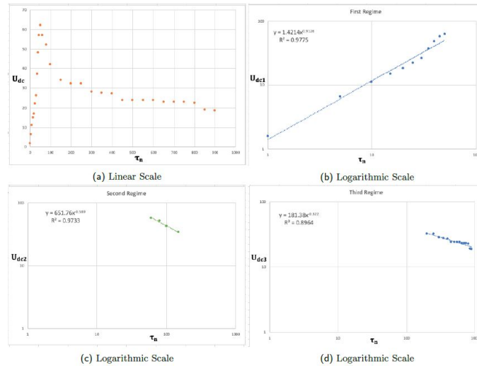
Fig. 5. Propagation speed of the Density current U_{dc} for the different Regimes with respect to time \tau_n at barrier position 0.28L/14 .
