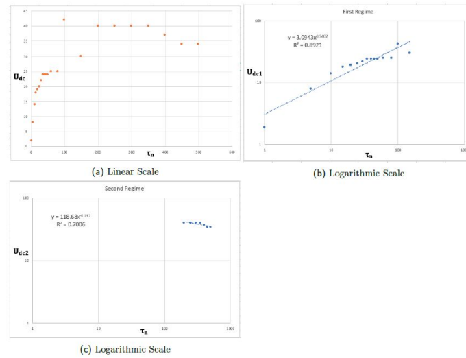
Fig. 13. Propagation speed of the Density current U_{dc} for the different Regimes with respect to time \tau_n at barrier position 1.68L/14 .
