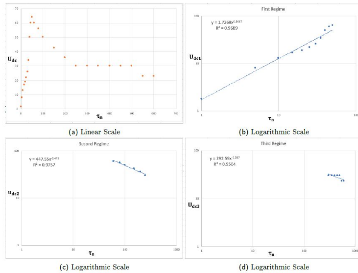
Fig. 6. Propagation speed of the Density current U_{dc} for the different Regimes with respect to time \tau_n at barrier position 0.42L/14 .
