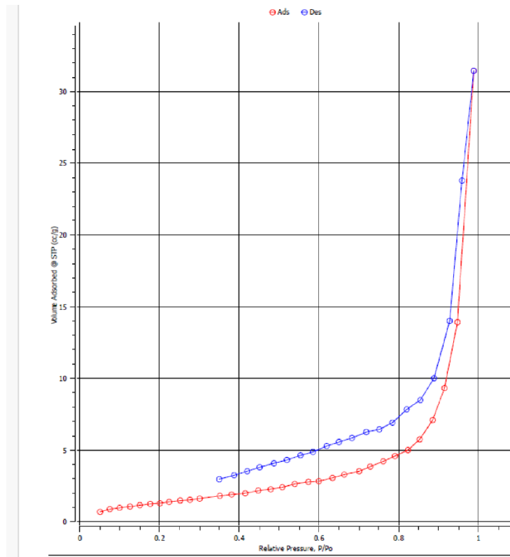
Fig. 8. BET adsorption isotherm- a
