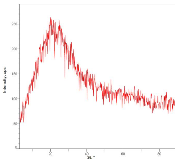
Fig. 5. XRD spectra of iron NP- a
