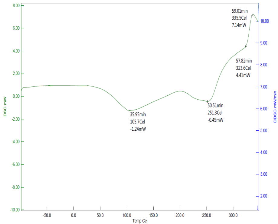
Fig. 7. DSC thermogram of iron NP
