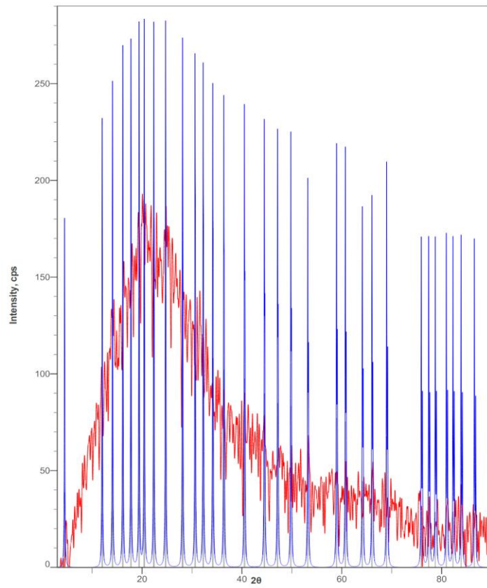
Fig. 6. XRD spectra of iron NP- b
