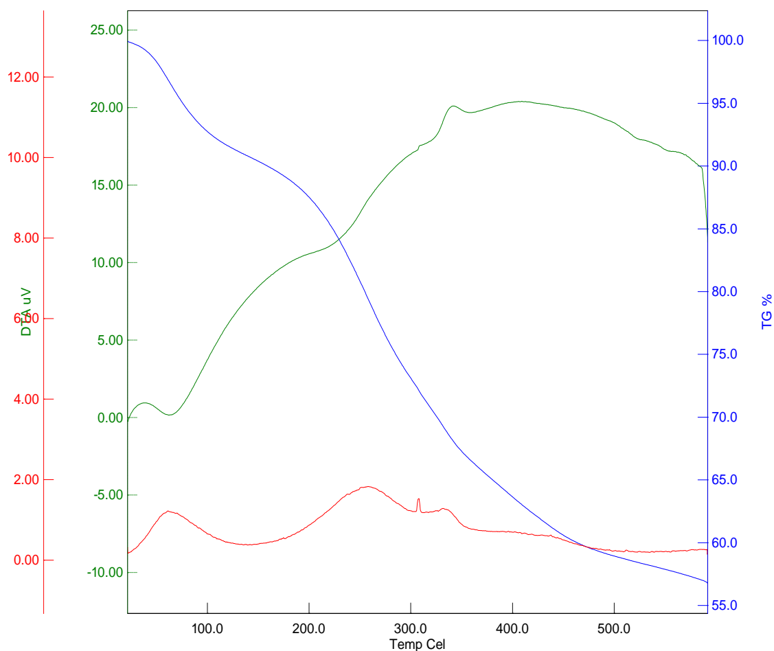
Fig. 10. TGA curve (using C. bicolor extract synthesized via aqueous)
