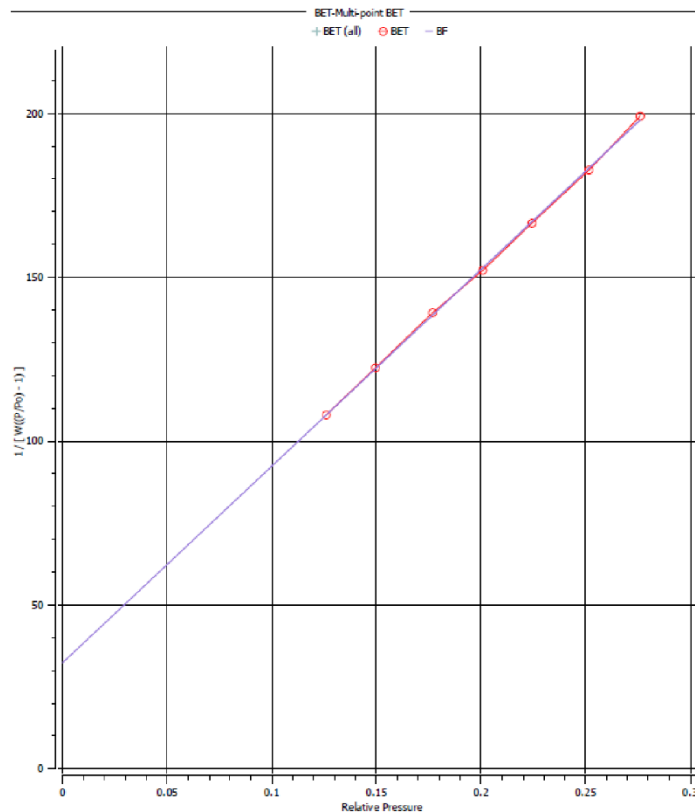
Fig. 9. BET adsorption isotherm - b
